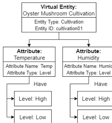
Figure 4. Information model for automatic monitoring system
