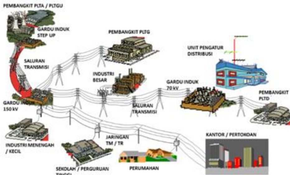
Gambar 1. Sistem Distribusi
