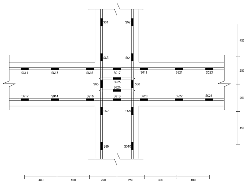
Figure 4. Strain Gauges Setup of The Specimen
