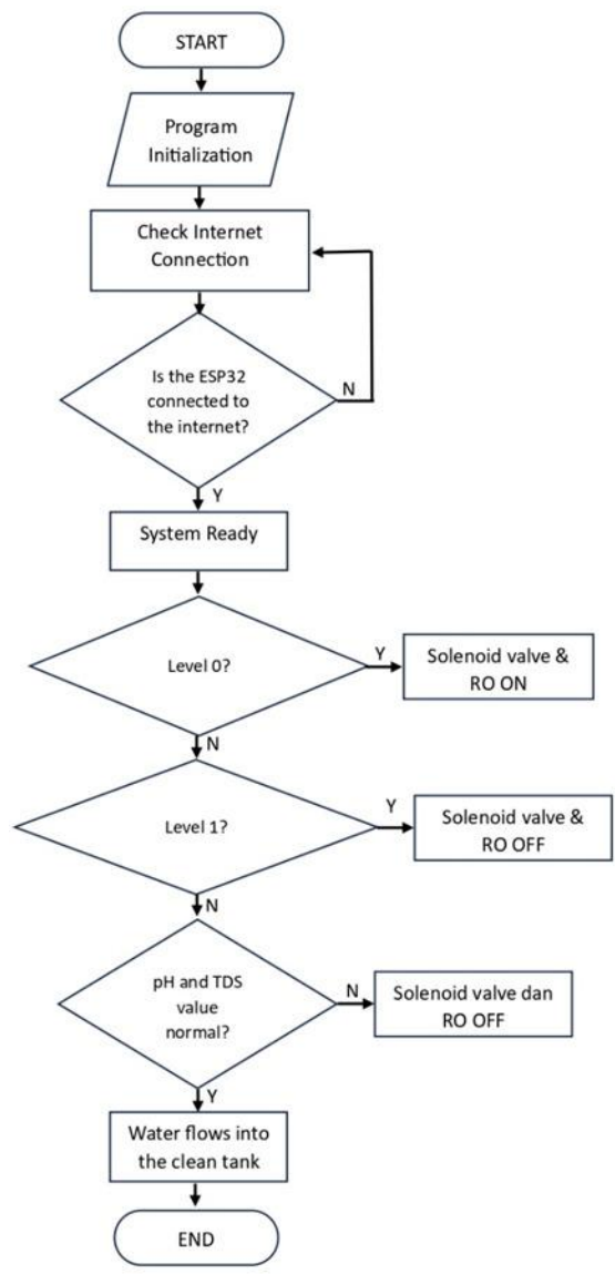
Figure 3. Flowchart of clean water tank system
