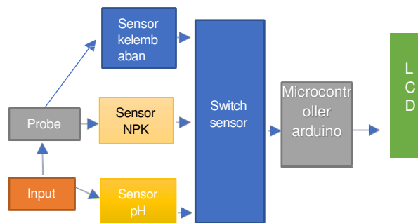
Gambar 2 Alur sensor
