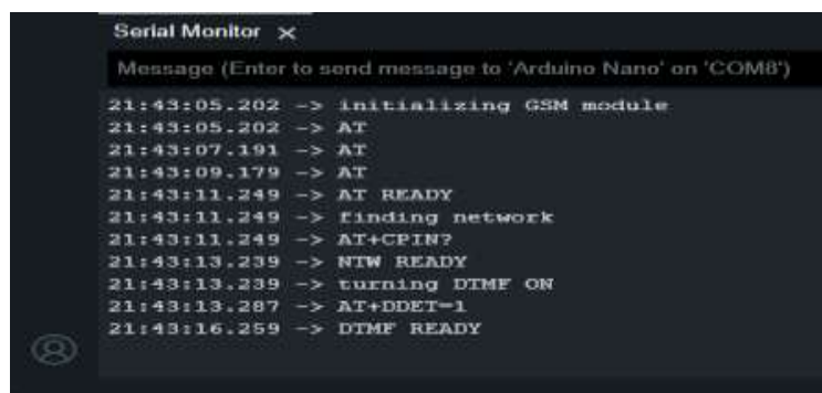
Gambar 8. Hasil serial monitor arduino IDE
