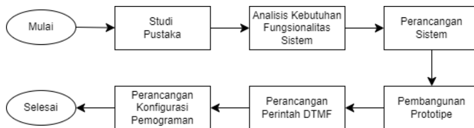
Gambar 1. Flowchart metodologi
