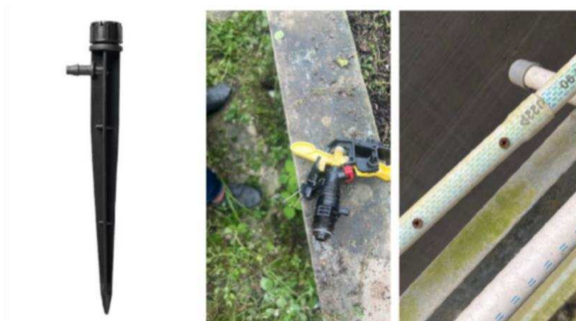
Figure 3 Prototype testing of irrigation components and the development of a low-cost screw adjusted pipe system as a frugal innovation for efficient water management.
