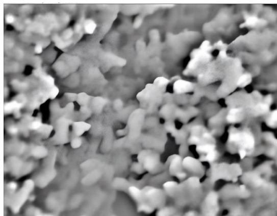
Fig 4. Scanning Electron Microscopy Result Section for Image J Analysis
