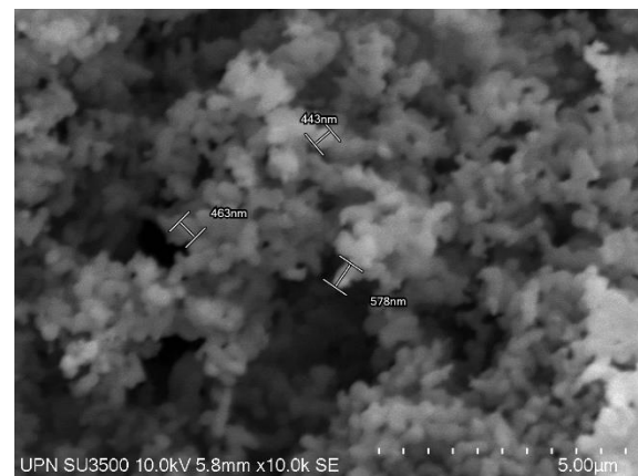
Fig 3. Scanning Electron Microscopy Results of Hydroxyapatite-Gelatin pH 10 30% Concentration with 10,000x Magnification.
