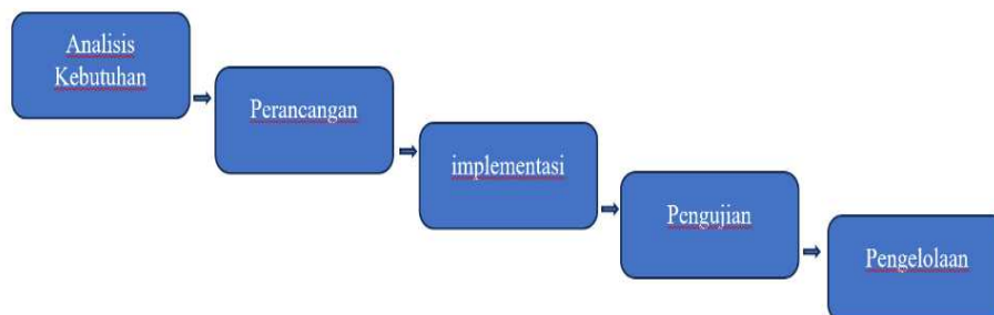
Gambar 1. Metode Waterfall
