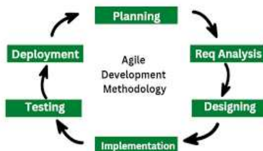
Gambar 1. Agile method
