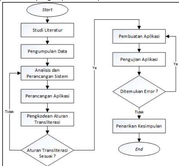
Gambar 6. Alur penelitian.
