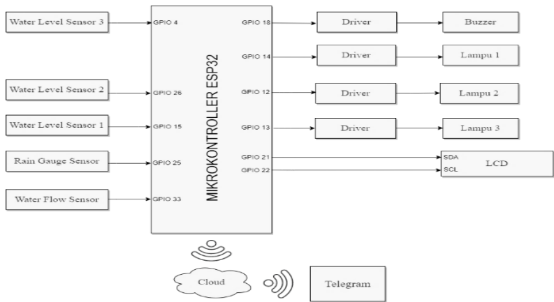
Gambar 1. Blok Diagram
