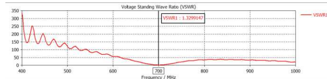
Gambar 10 VSWR
