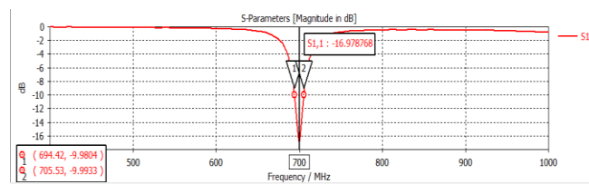
Gambar 9 Return Loss
