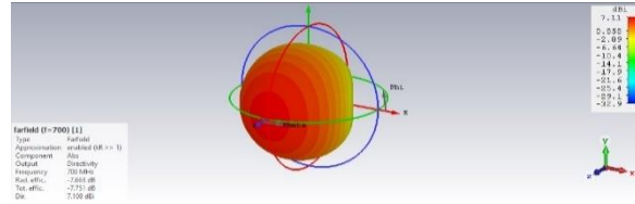
Gambar 12 Gain antenna
