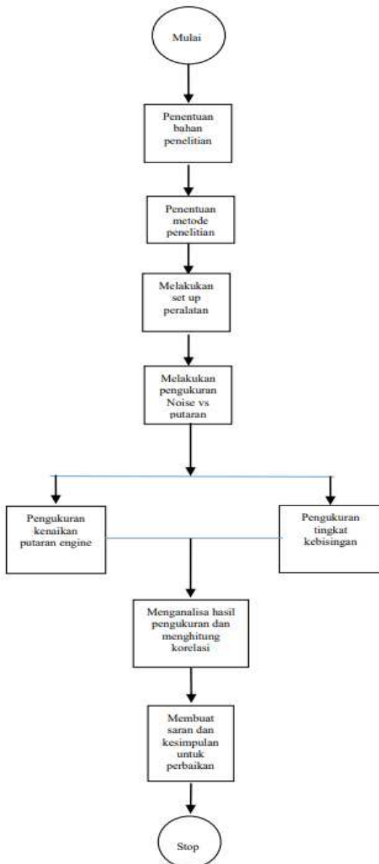
Gambar 3. Alur Penelitian
