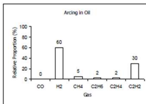
Figure 4. Arcing in oil
