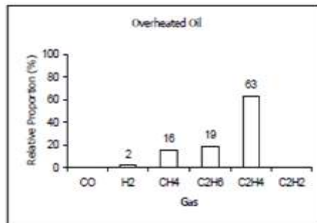
Figure 1. Oil overheating
