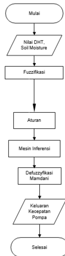
Gambar 2. Flowchart Sistem
