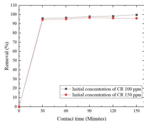
Fig 3. Effect of contact time and initial dye concentration on the adsorption of CR dye with Chi-FA-Fe 3 O 4 composite adsorbent
