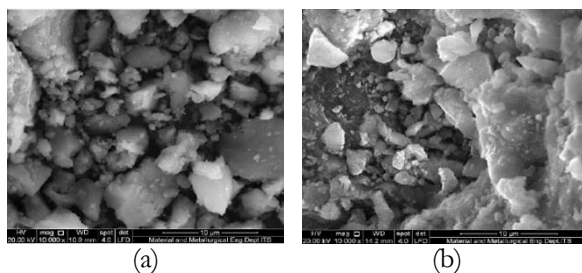
Fig 2. SEM analysis with 10,000x magnification (a) Chi-FA-Fe 3 O 4 composite and (b) Chi-FA-Fe 3 O 4 composite after adsorption of CR dye
