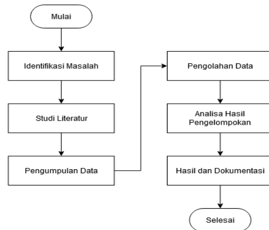
Gambar 1. Metode Penelitian
