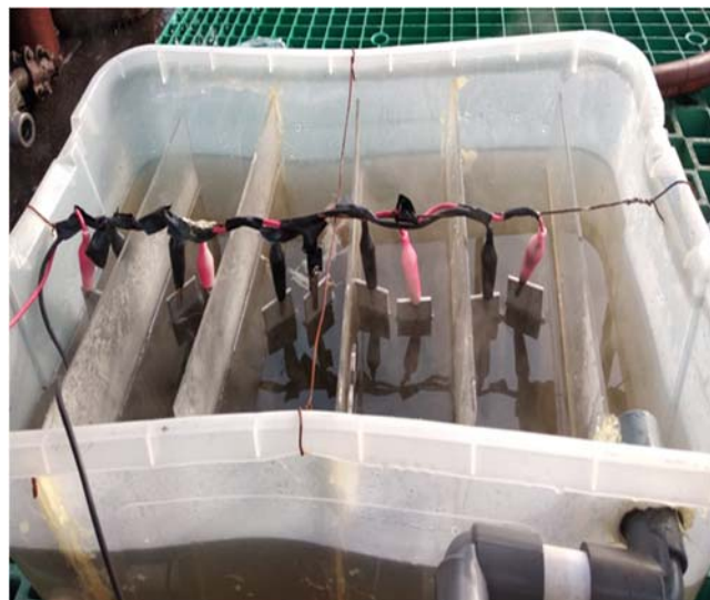
Figure 2. Modification of Ammonia Liquid Waste Management Device Design
