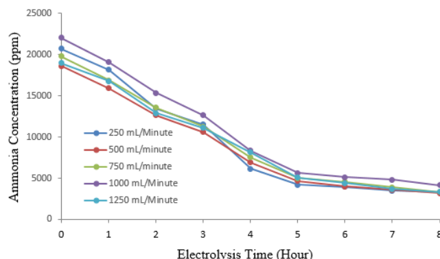
Figure 5. Curve effect of flow rate during electrolysis time
