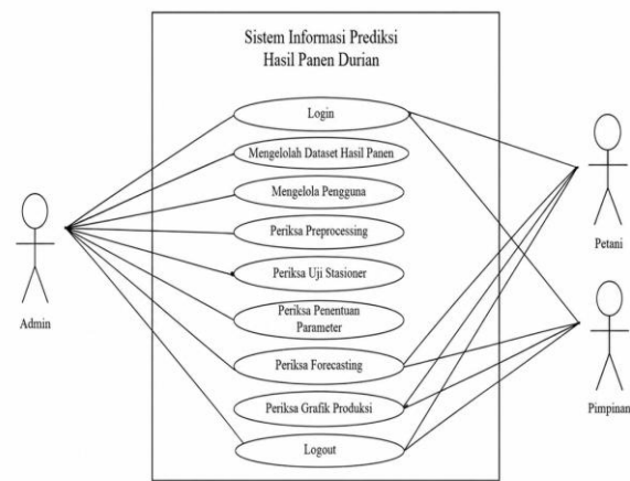
Figure 3. UML Use Case Diagram of Proposed Streamlit Forecasting System
