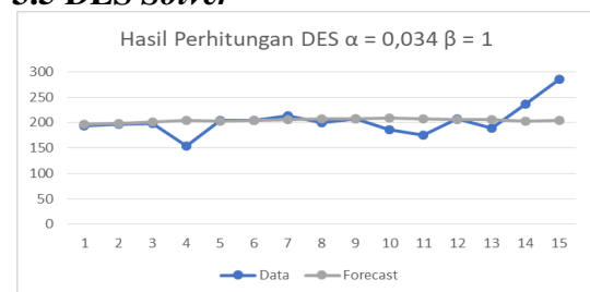
Gambar 7. Double Exponential Smoothing Solver
