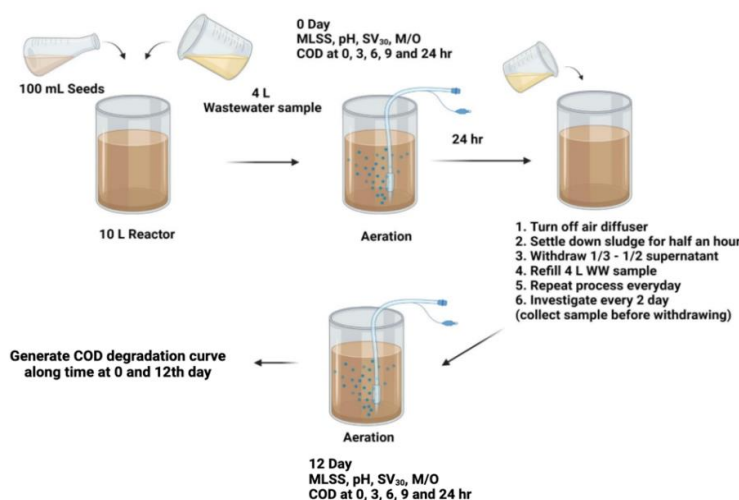
Figure 1. Aerobic degradation test
