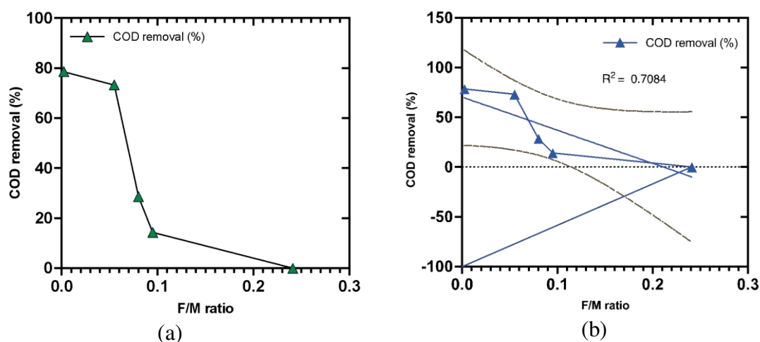
Figure 6. Effect of F/M ratio to COD (mg/L) (a) Effect of F/M ratio on COD removal (b) Linear regression analysis of the effect of F/M ratio on COD removal
