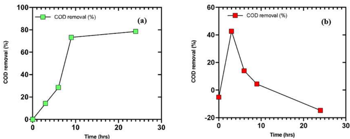
Figure 4. COD removal efficiency (a) on day 0 (b) on day 12
