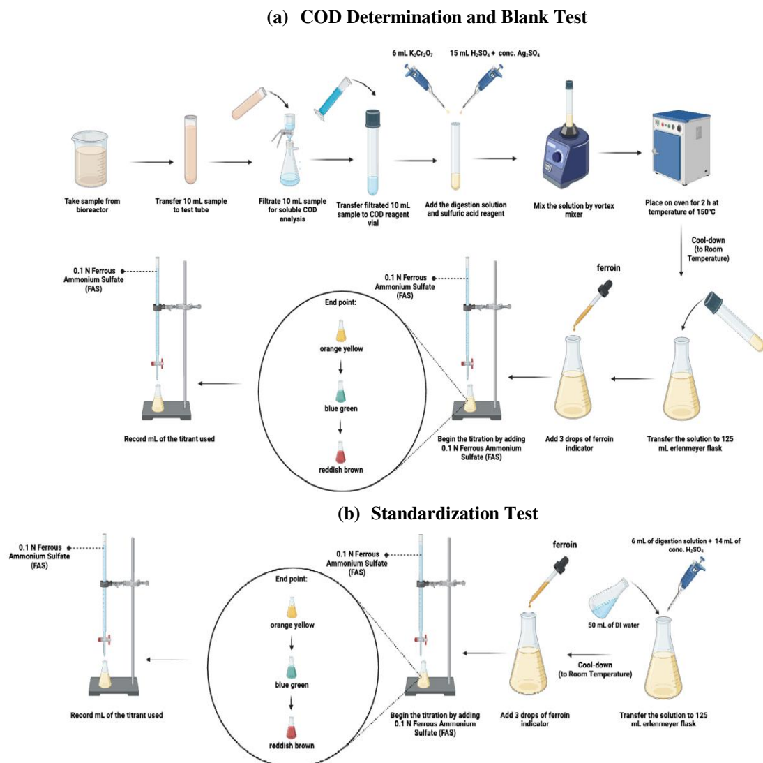
Figure 2. COD determination by closed reflux titrimetric method: (a) COD determination and blank test and (b) standardization test
