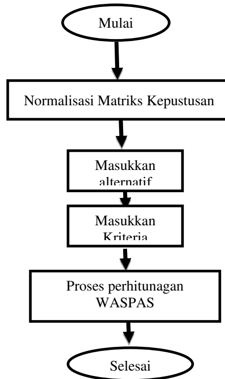
Gambar 2.1. Flowchart metode WASPAS
