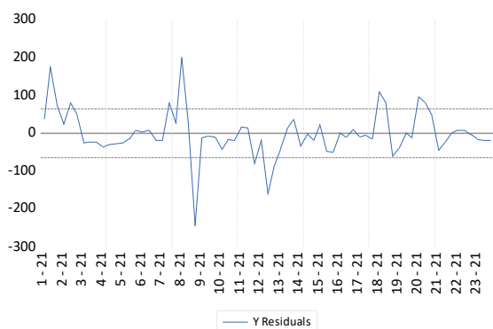
Figure 3 Heteroscedasticity Test Result Source : Processed by researchers, (2025)
