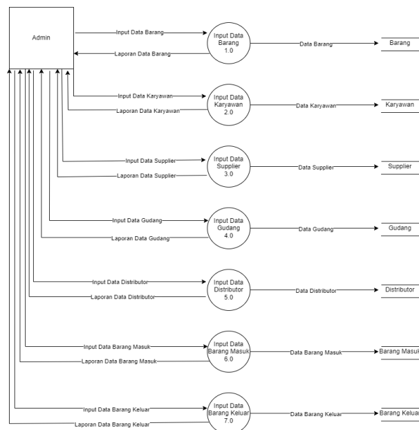
Gambar 9. Diagram Nol
