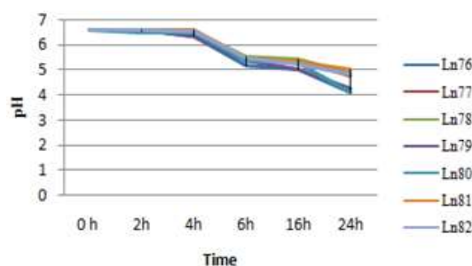
Figure 2. Production of lactic acid by some subspecies (correlation between pH condition and Incubation time). Samples for Mesenteroides are shown in Ln76, Ln77, and Ln78. Samples for Dextranicum are shown in Ln79 and Ln80. Samples for Cremoris are shown in Ln81 and Ln82.
