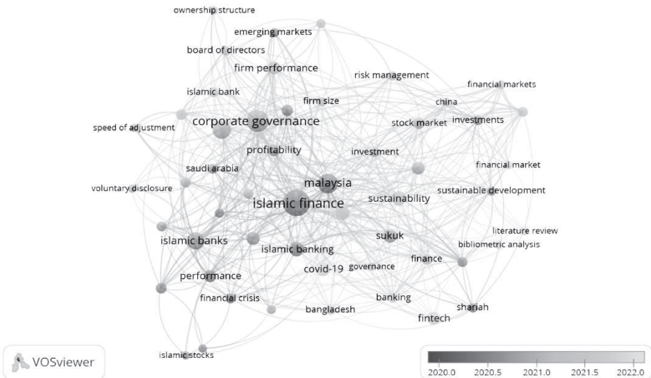
Figure 4. Keyword Co-occurrence Network
