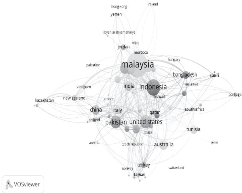
Figure 2. Visualization of Co-Authorship among Countries
