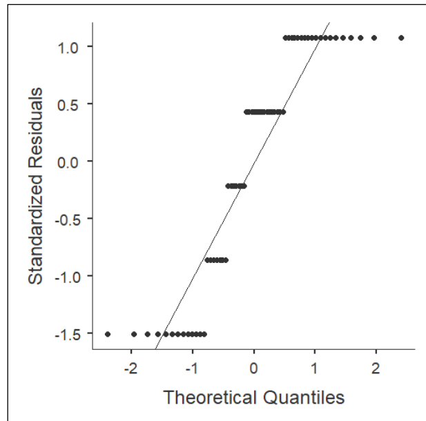
Figure 3. Q-Q Plot
