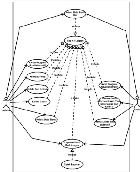
Gambar 3. Usecase Diagram
