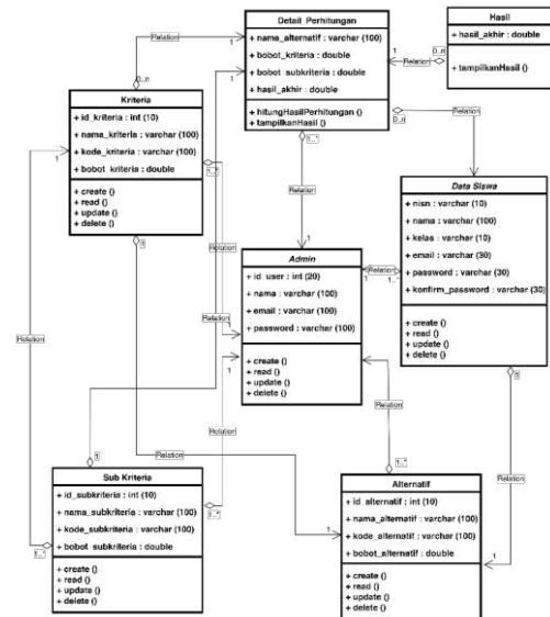
Gambar 4. Class Diagram
