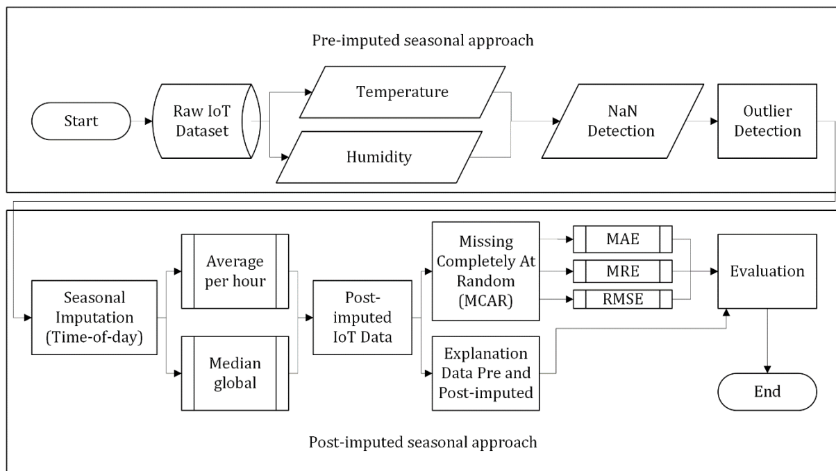
Figure 1. Pre- and Post-Imputed Seasonal Methodology
