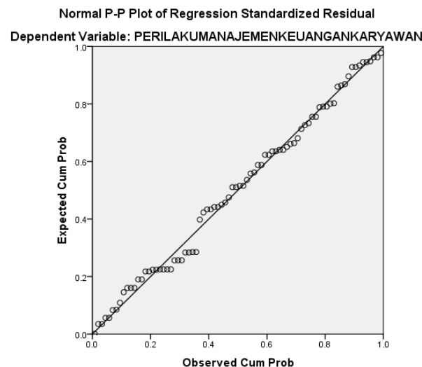
Gambar 1 Scatterplot
