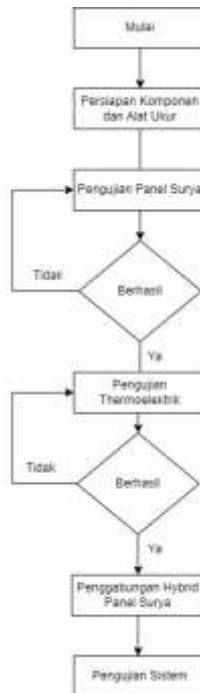
Gambar 5 Diagram Penelitian
