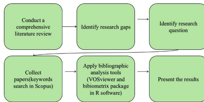
Figure 2. Study's framework.
