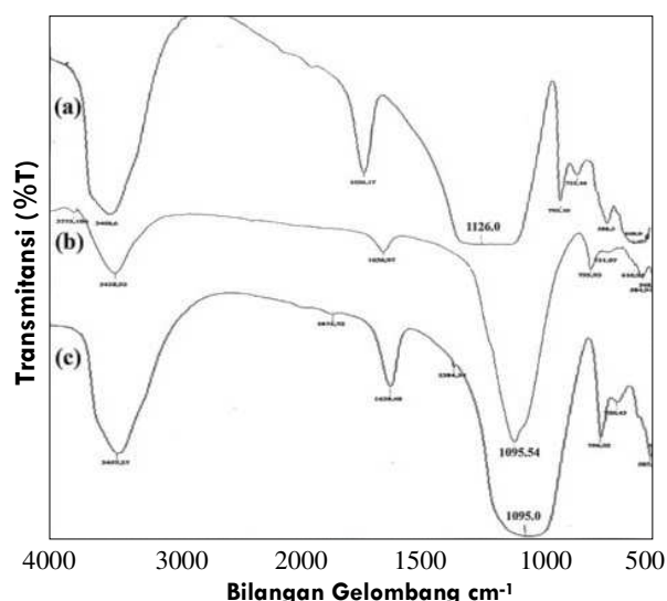
Gbr 1. Spektra IR(a) ZA, (b) ZAA, (c) CuO/ZAA
