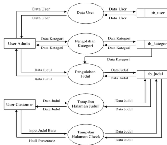
Gambar 3 Perancangan Data Flow Diagram (DFD) Level 1
