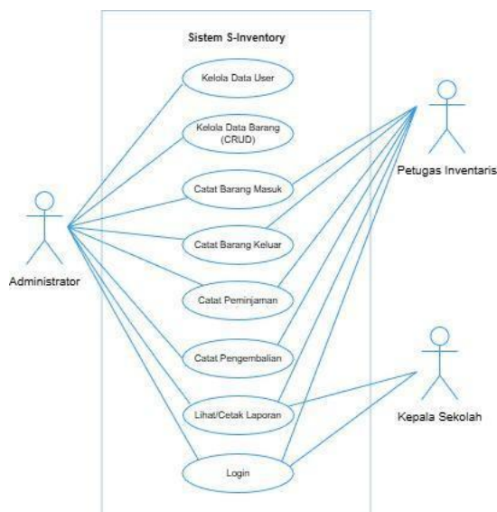
Gambar 2. Use Case Diagram Sistem S-Invento
