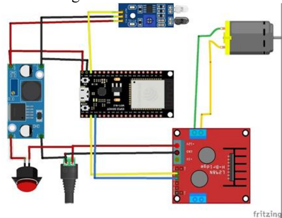
Figure 8. Product Wiring Design (Source: Author documentation, 2024)
