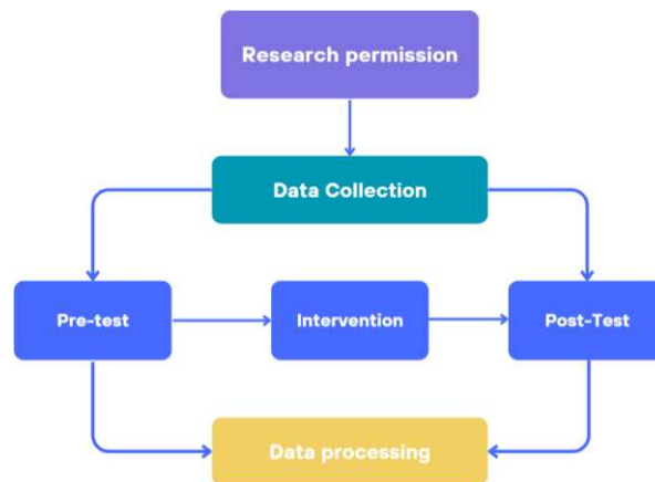
Figure 1. Research flow
