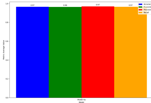
Fig. 8. Confusion values in average Values of Model 4.
