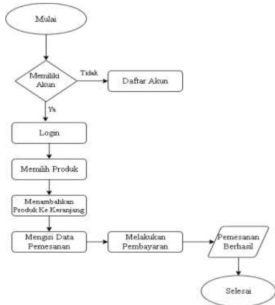
Gambar 1. Flowchart Sistem Usulan
