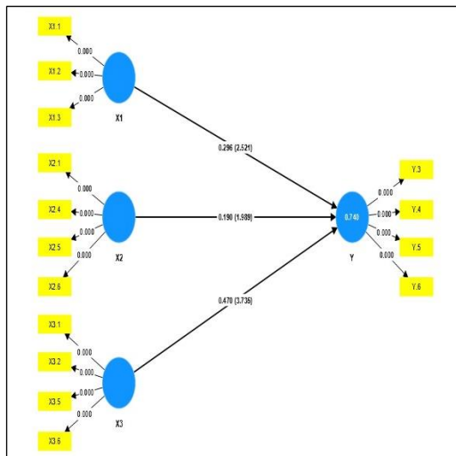
Gambar 1: Model Penelitian
