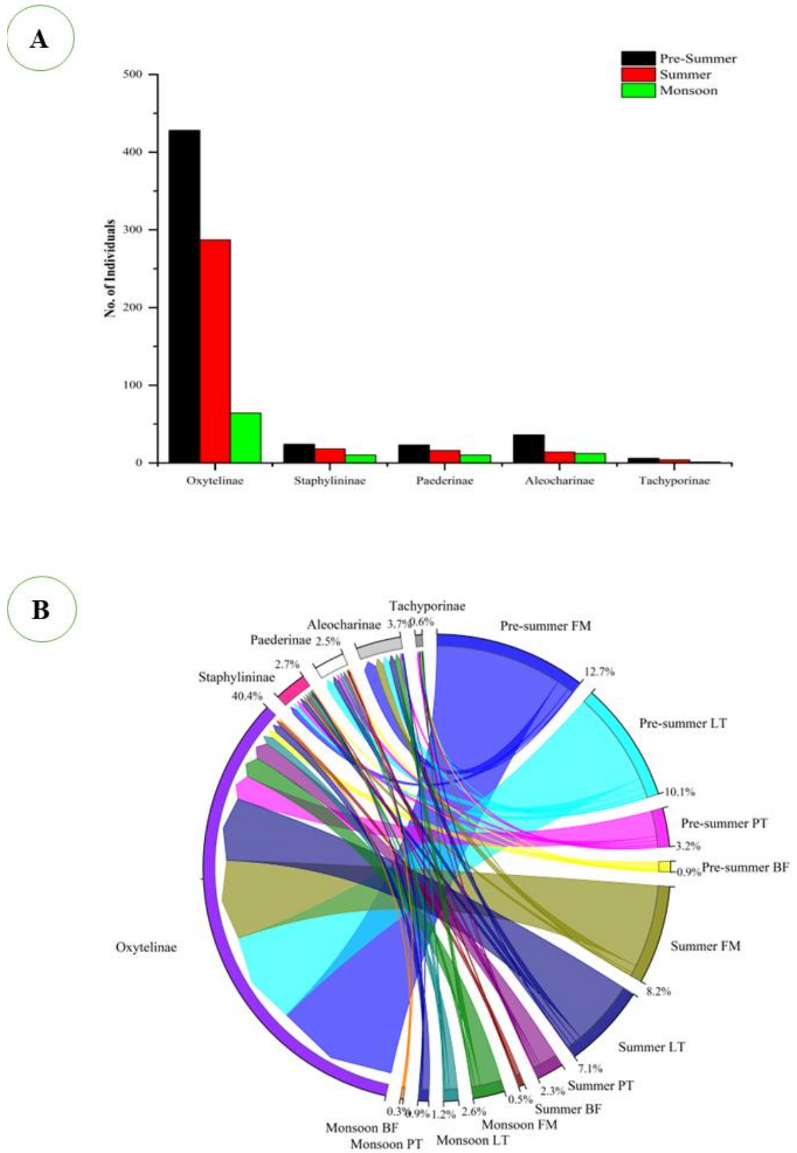
Figure 4. Akalapuzha mangrove coastal ecosystem (A) Diversity, and seasonal variation; (B) correlation between seasonal variation and diversity
