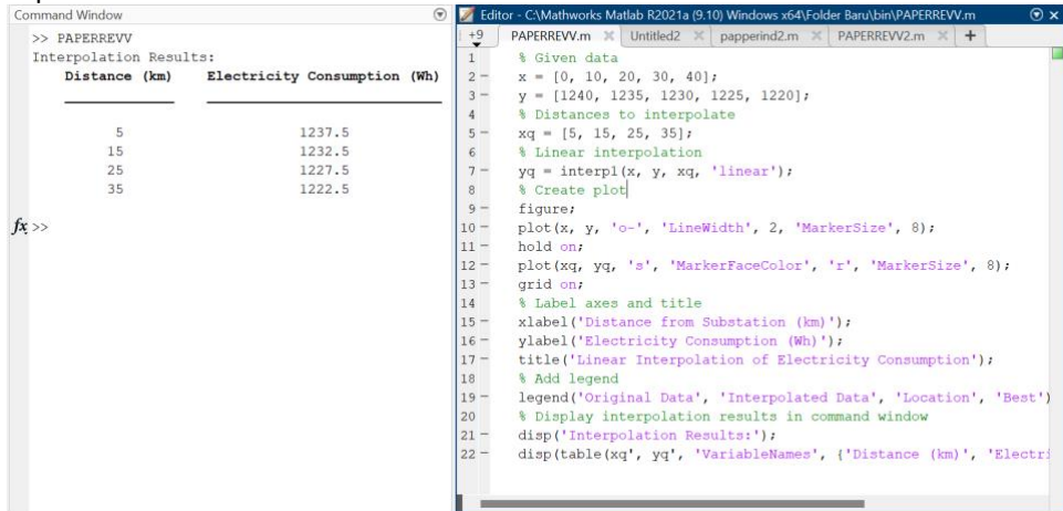
Figure 1. Matlab implementation of the Linear Interpolation Method
