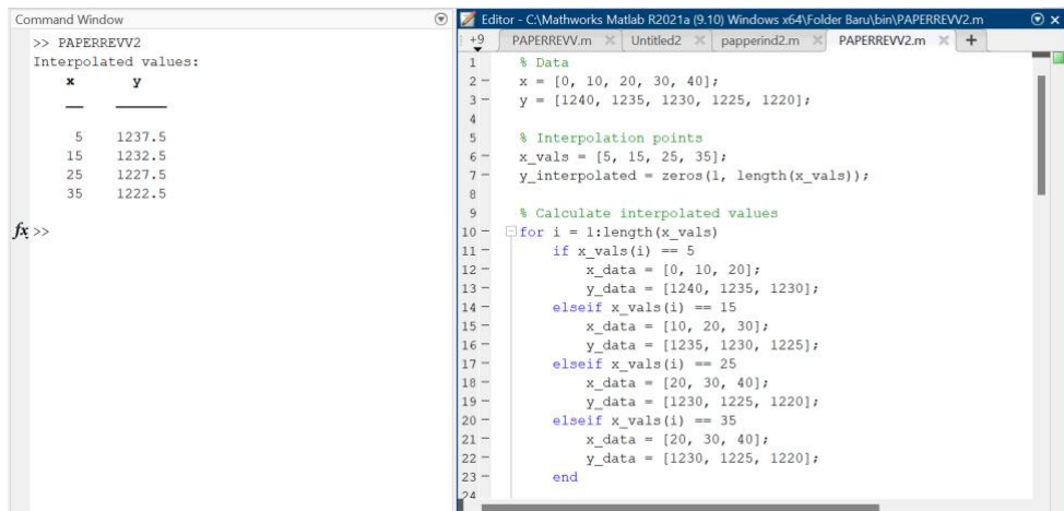
Figure 2. Matlab implementation of the Quadratic Interpolation Method
