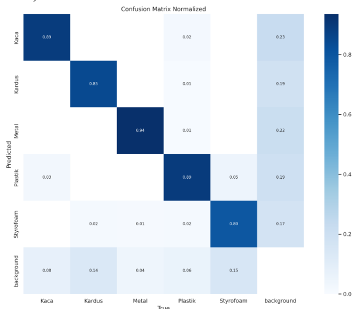
Gambar 9 Confusion Matrix
