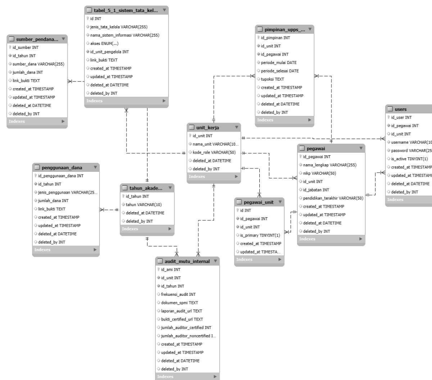
Gambar 6. Entity Relationship Diagram (ERD) Kriteria 1
