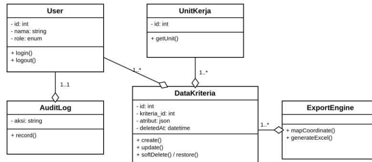
Gambar 5. Class Diagram Sistem
