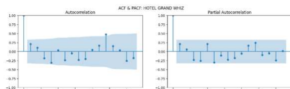
Figure 8. ACF and PACF Plots of Hotel Grand Whiz
