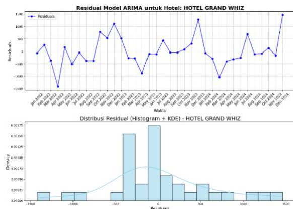
Figure 14. Diagnostic Checking Hotel Grand Whiz
