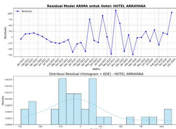
Figure 16. Diagnostic Checking Hotel Arrayana
