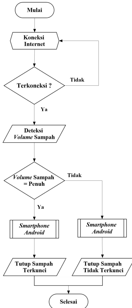
Gambar 2. Flowchart Sistem
