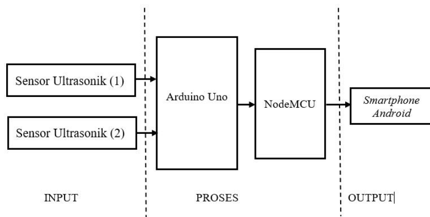
Gambar 1. Blok Diagram
