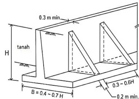
Gambar 4. Dinding penahan tanah tipe buttress Sumber: Hardiyatmo, 2020
