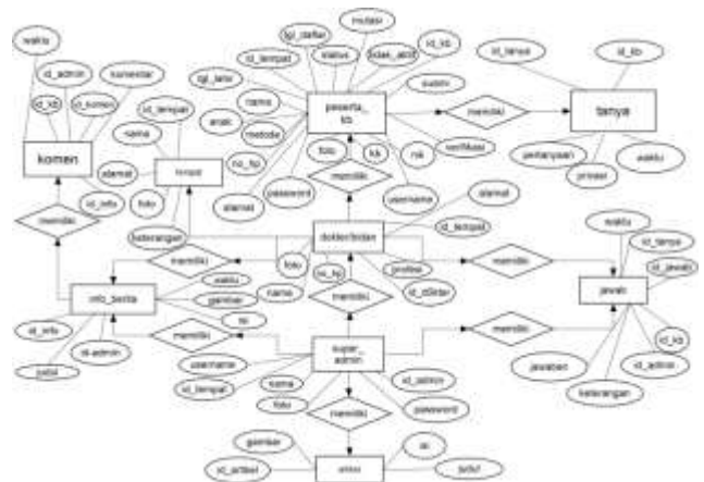
Gambar 3 Entity Relationship Diagram (ERD)
