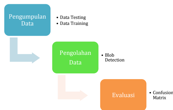
Gambar 1. Alur Penelitian
